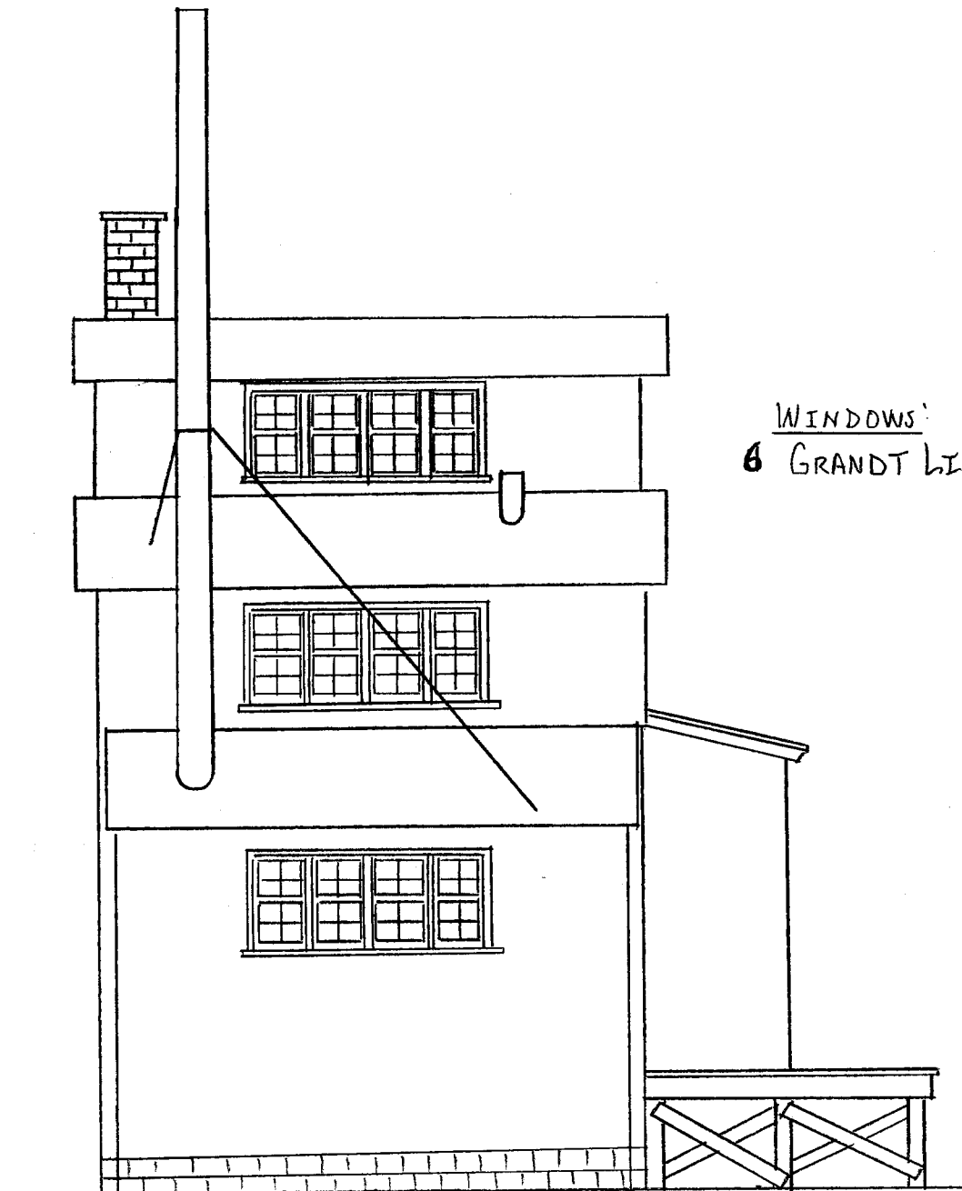
LEFT ELEVATION H.O. SCALE
